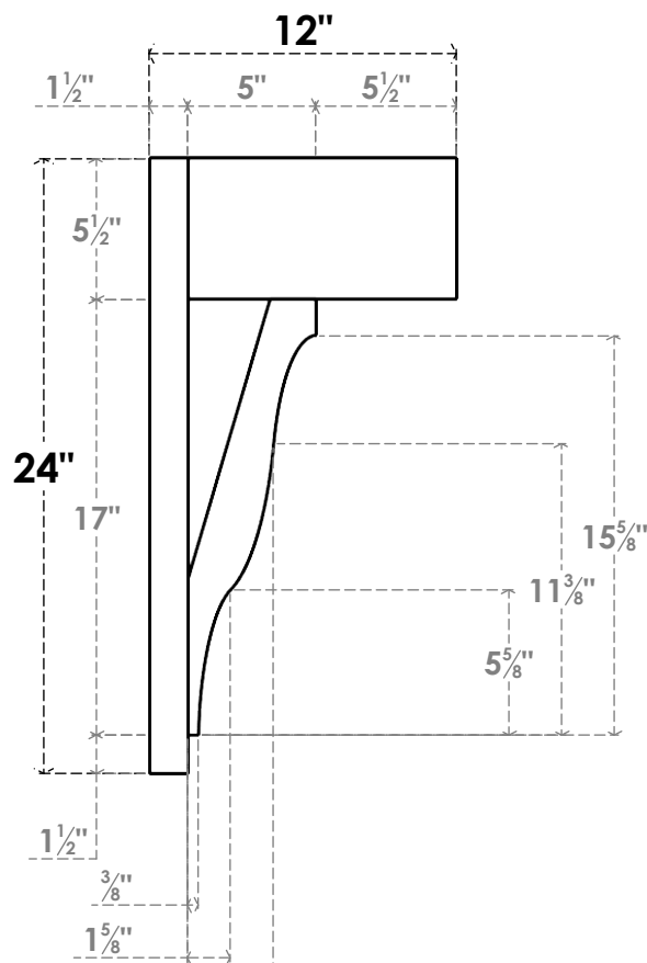
SIDE PROFILE
